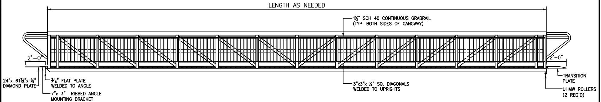
ELEVATION VIEW OF ALUMINUM GANGWAY
